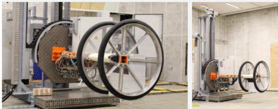
Propulsion test facility with a double propulsion unit
